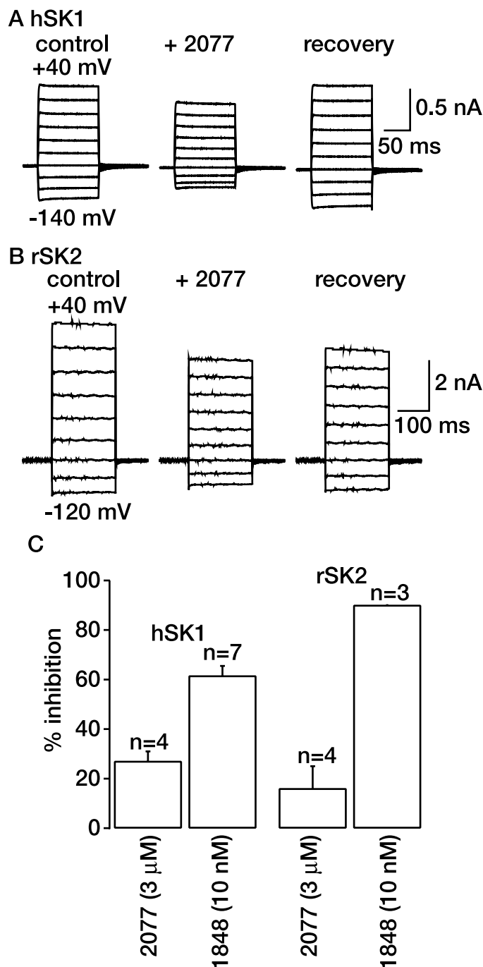
Fig. 3. Effects of UCL2077 on SK currents. Example traces of hSK1 (A) and rSK2 (B) currents in the absence, presence, and washout of 3 \mu\text{M} UCL2077. The currents were elicited by 100- to 200-ms steps from -120/-140 mV to +40 mV from a holding potential of -80 mV. C, summary of effects of 3 \mu\text{M} UCL2077 and 10 \text{ nM} UCL1848 on SK currents. The numbers of observations for each treatment are shown above the bar.
